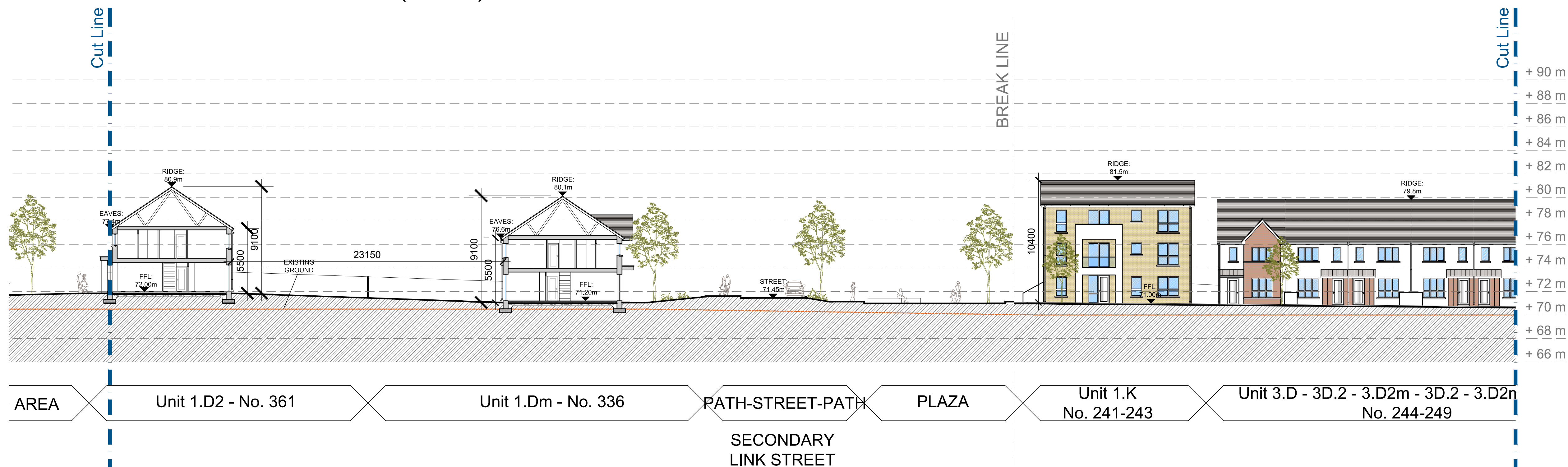
PROPOSED SITE SECTION BB (Part 2) - scale 1:200
