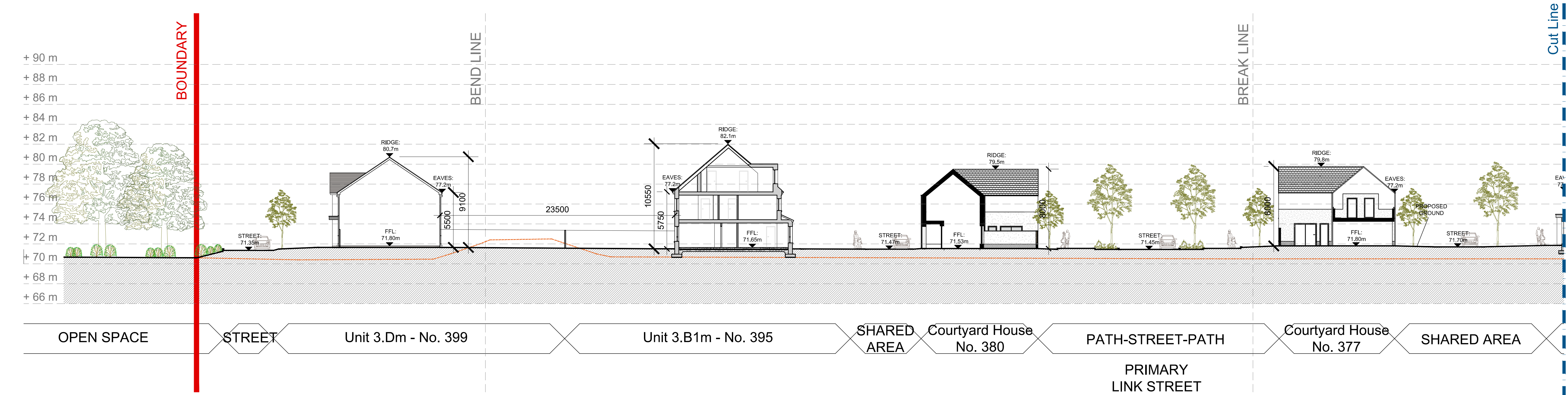
PROPOSED SITE SECTION BB (Part 1) - scale 1:200
